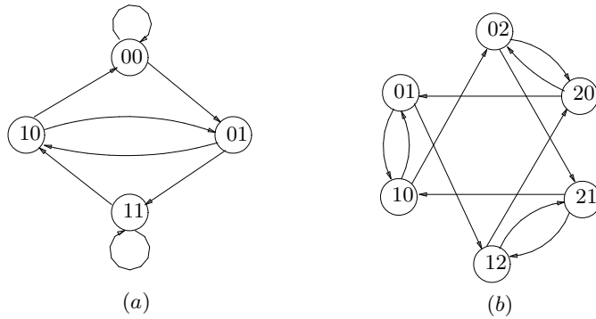
Figure 4.6 (a) The de Bruijn digraph D_B(2, 2) ; (b) The Kautz digraph D_K(2, 2) .
