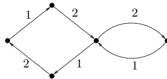
Figure 11.9 Weakly eulerian non-eulerian 2-arc-coloured digraph.
