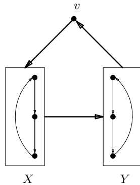
Figure 7.20 A strong tournament T on 7 vertices. The fat arcs indicate that all arcs between the sets indicated have the directions shown.
