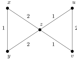
Figure 11.4 A non-convenient 2-edge-coloured graph.
