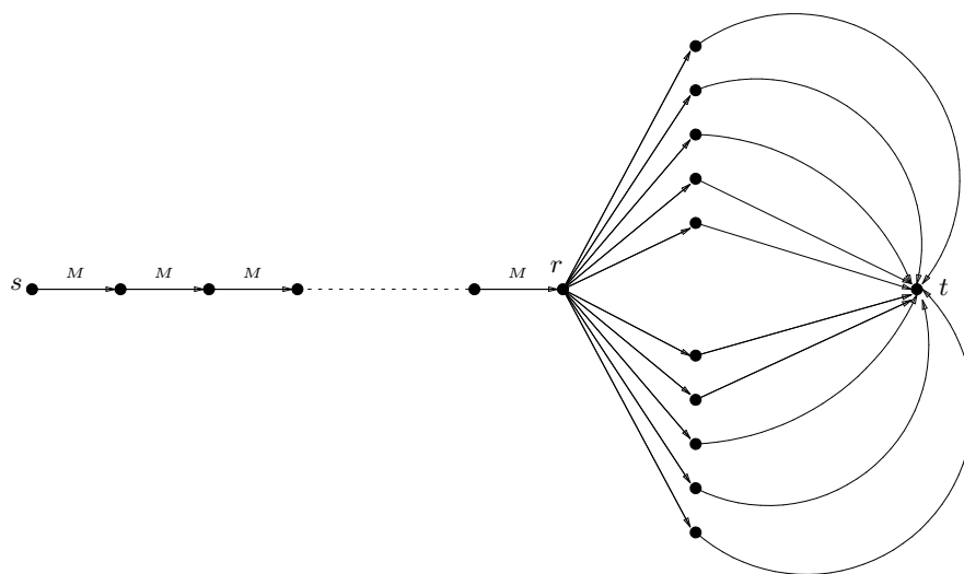
Figure 3.11 A bad example for a standard flow algorithm such as the Edmonds-Karp algorithm. The capacities of arcs are either 1, if no number is shown or M , where M is a large number. Algorithms such as the Edmonds-Karp algorithm will augment M times along the path from s to r each time by just one unit.
