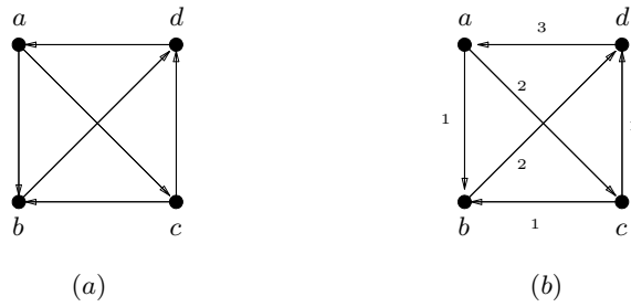
Figure 3.20 Part (a) shows a digraph with cost 1 (not shown) on every arc. Part (b) shows the values of a minimum cost circulation in the corresponding network. This circulation corresponds to the postman tour abdacdbda .
