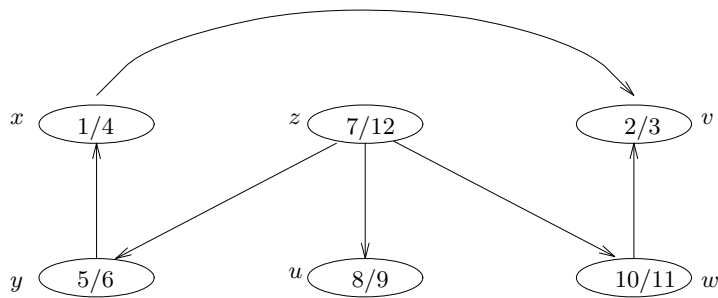
Figure 4.2 The result of applying DFSA to an acyclic digraph
