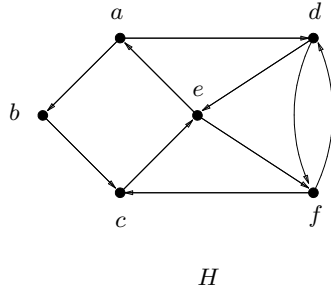
Figure 1.11 A digraph H .
