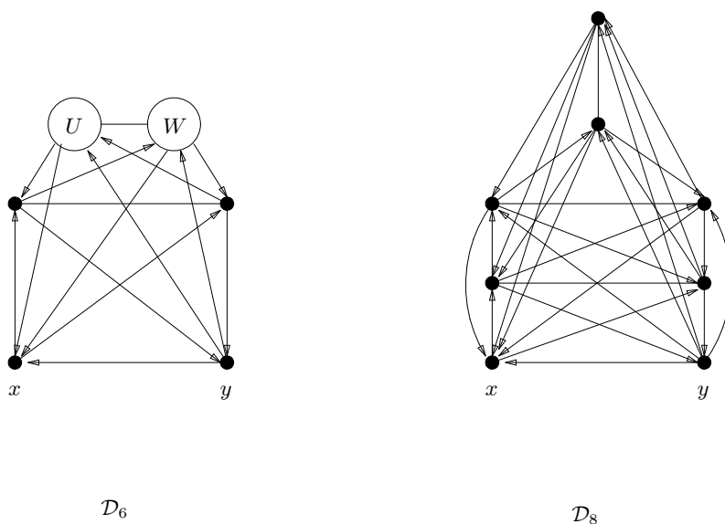
Figure 6.3 The two families of non-arc-pancyclic arc-3-cyclic tournaments. Each of the sets U and W induce an arc-3-cyclic tournament. All edges that are not already oriented may be oriented arbitrarily, but all arcs between U and W have the same direction.
