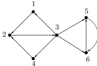
Figure 5.8 The digraph L .
