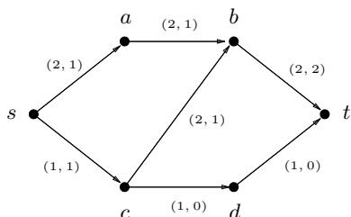
Figure 3.9 A network \mathcal{N} with flow x which is maximal but not maximum as the path P = sabc dt is an (s, t) -path in \mathcal{N}(x) . Note that the arc bc is a backward arc of P . The data on each arc are (capacity, flow).
